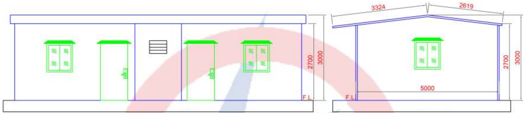
FRONT ELEVATION
