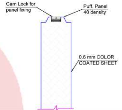
PANEL DETAIL
